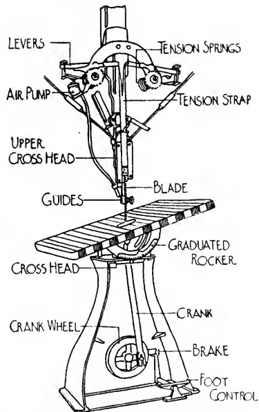
FIG. 190. SCROLL OR JIG-SAW.
